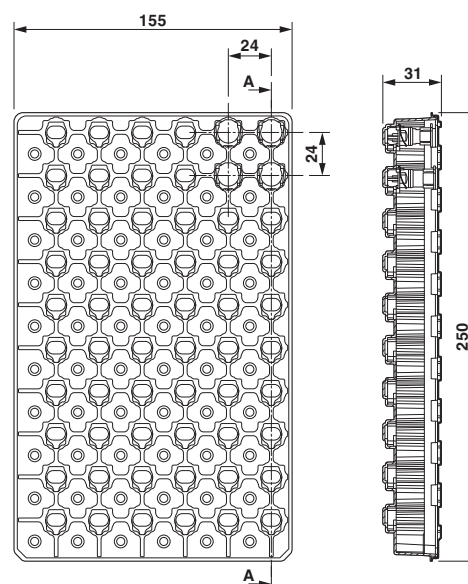
THR tray packaging
