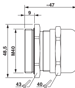
Dimensional drawing
