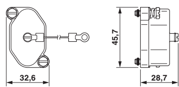
Dimensional drawing
