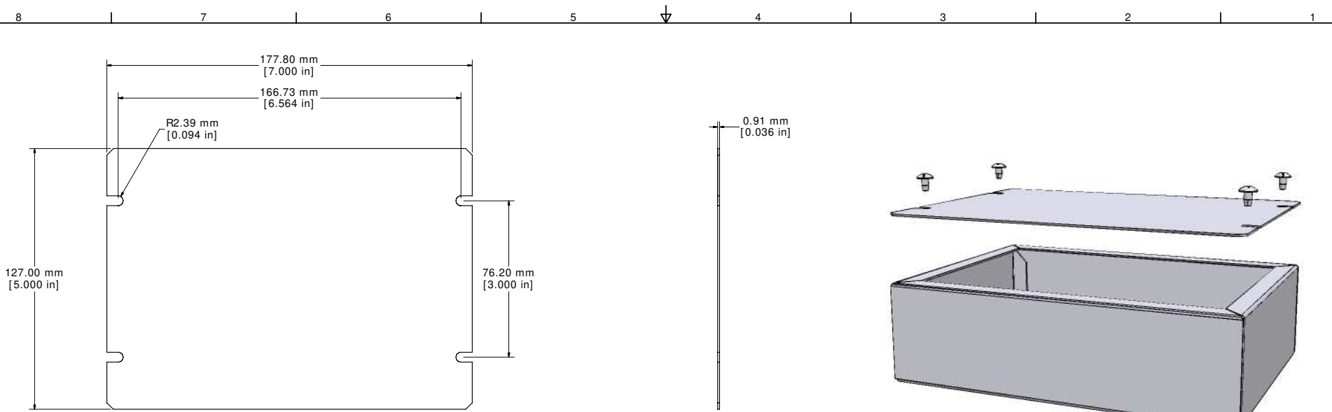
1431-12 OR 1431-12BK3 - VIEW FROM TOP (SOLD SEPERATELY)
