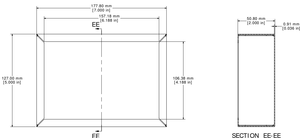
1441-12 OR 1441-12BK3 - VIEW FROM TOP (SOLD SEPERATELY)
