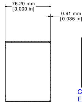
SECTION EE-EE
