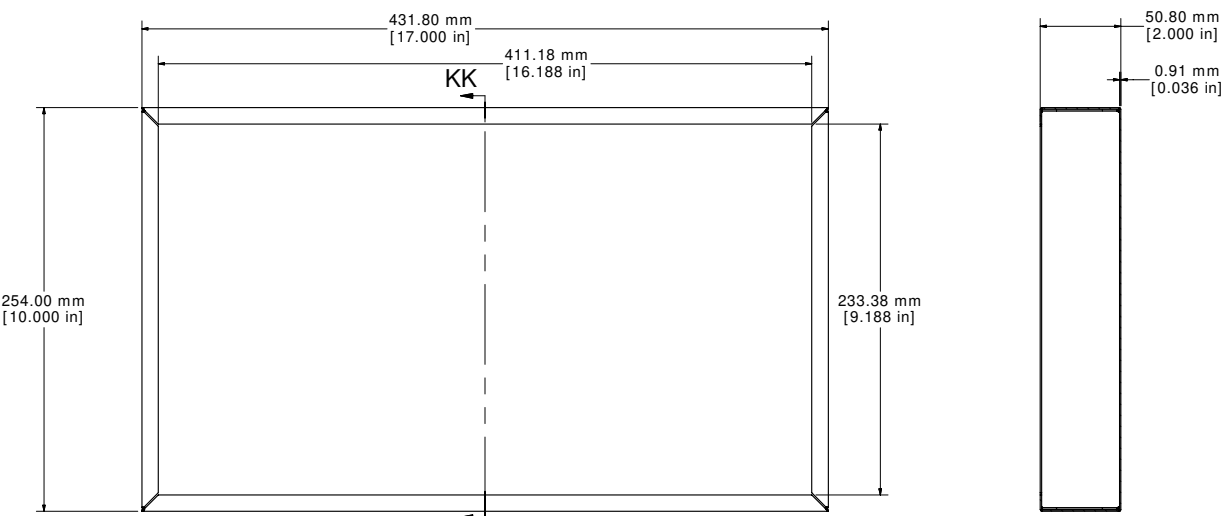
SECTION KK-KK
