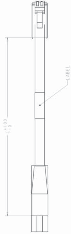
(CONNECTOR 1)
