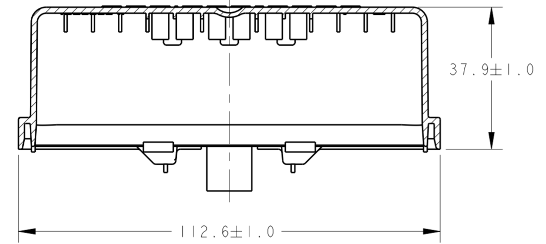
SECTION B-B
