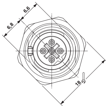
Dimensional drawing
