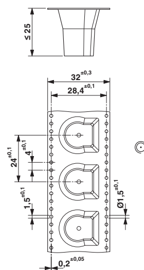
Dimensional drawing
