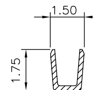
SEC C-C
