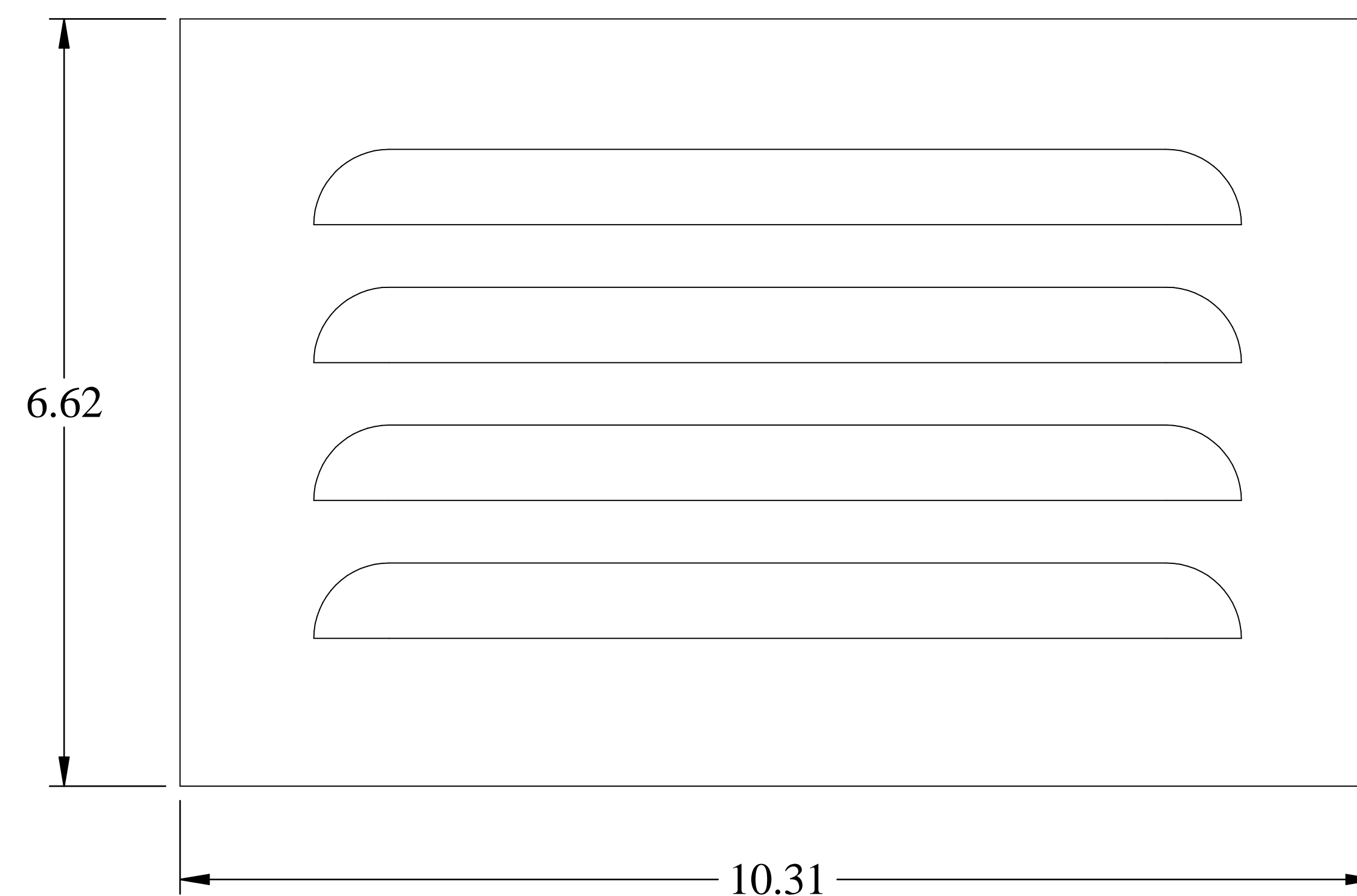
FRONT VIEW
