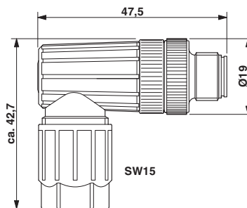
Dimensional drawing
