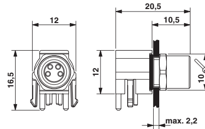
M8 flush-type socket
