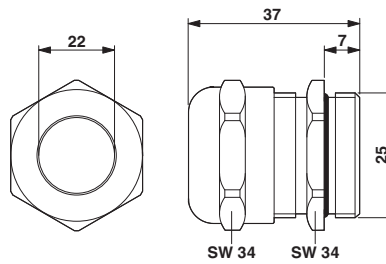
Dimensioned drawing
