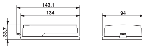
Dimensioned drawing
