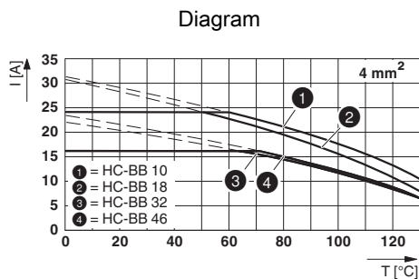
Derating diagram (conductor cross section: 4.0 mm 2 )
