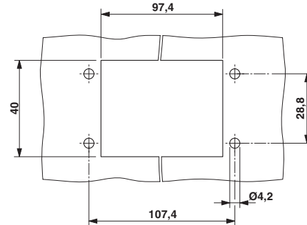
Mounting cutout for HC-B 24-ANDOCK-MOD...
