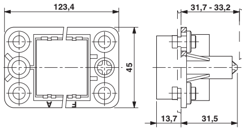
Dimensional drawing of HC-B 24-ANDOCK-MOD...
