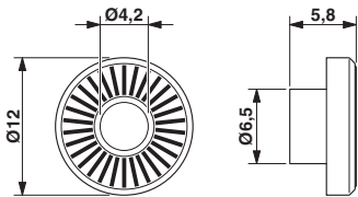
Dimensioned drawing
