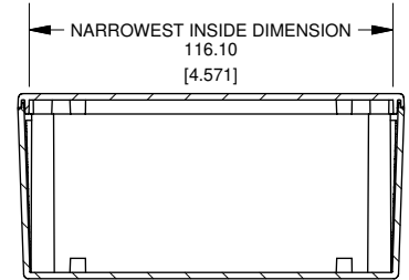
SECTION C-C
