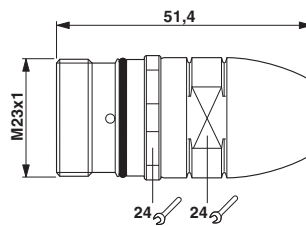
Dimensional drawing
