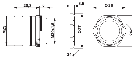
Dimensioned drawing
