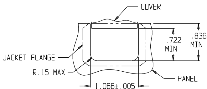
PANEL CUTOUT
