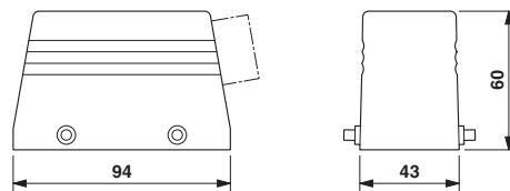
Dimensioned drawing
