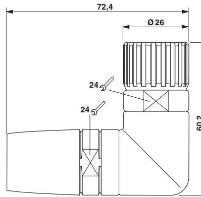
Dimensioned drawing
