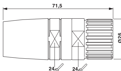
Dimensional drawing
