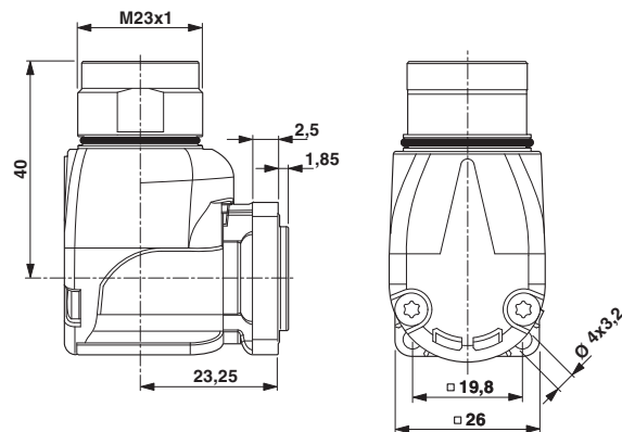
Dimensioned drawing
