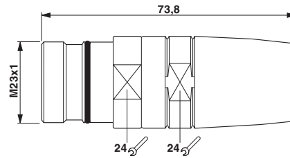
Dimensioned drawing
