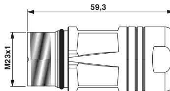
Dimensioned drawing
