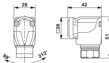
Dimensioned drawing
