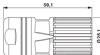
Dimensional drawing
