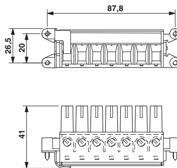
Dimensioned drawing
