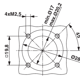
Dimensioned drawing
