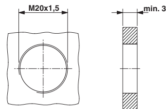
Dimensioned drawing
