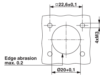
Dimensioned drawing
