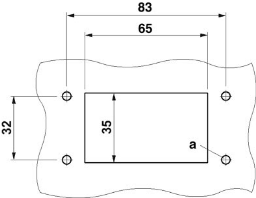
Panel cutout
