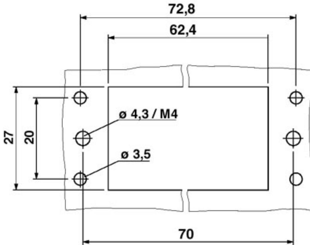
Panel cutout
