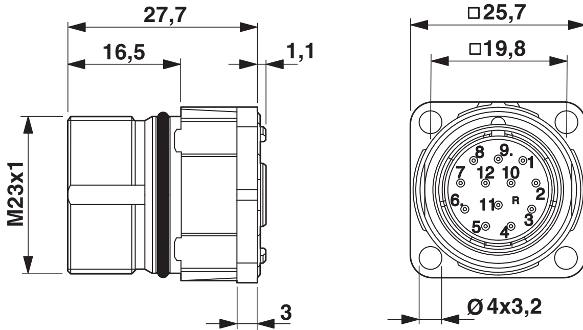
Dimensioned drawing
