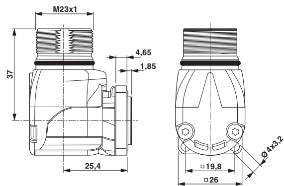
Dimensioned drawing
