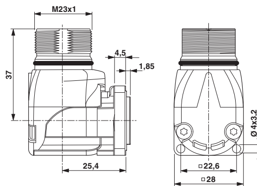
Dimensioned drawing
