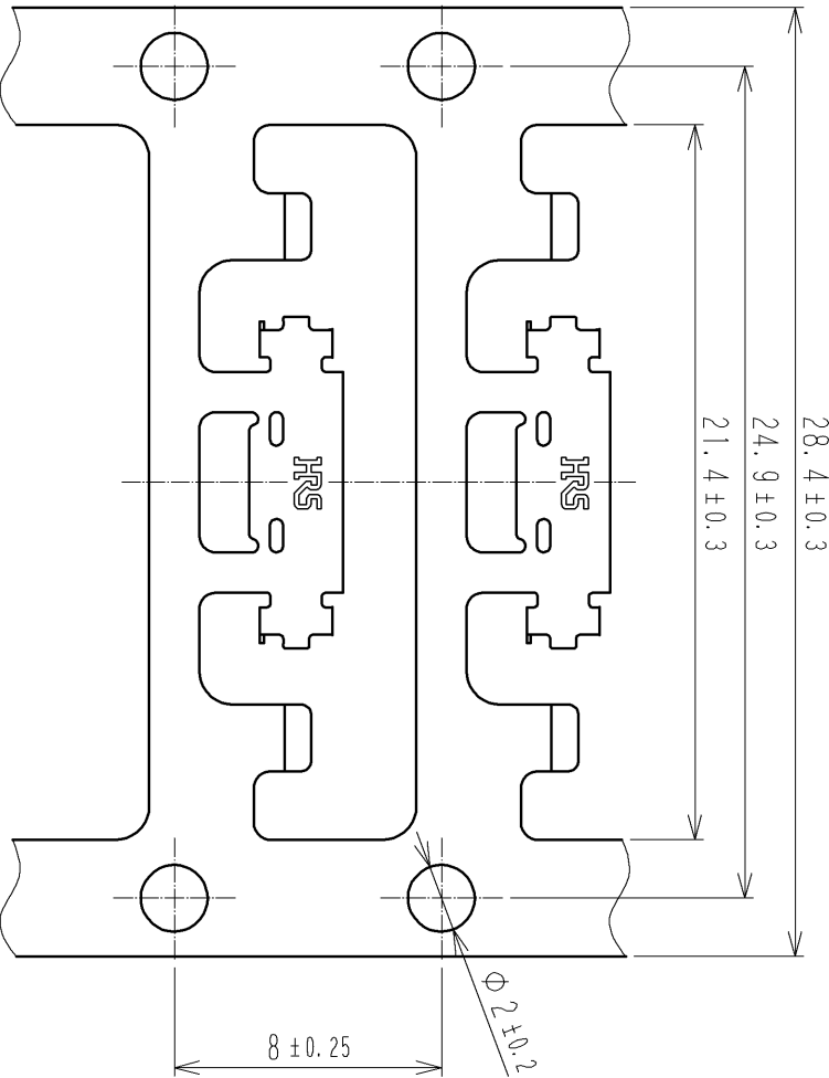
CARRIER STATE DRAWING(FREE)
