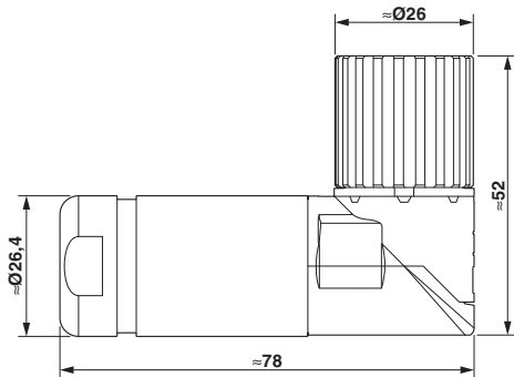
Dimensional drawing
