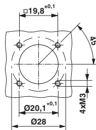
Dimensional drawing
