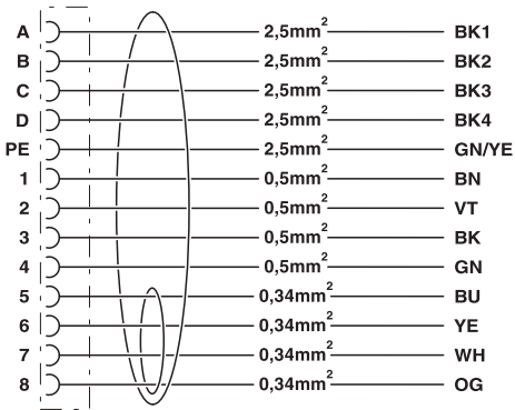
Circuit diagram
