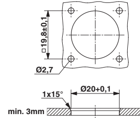
Installation dimensions Flat gasket, radial O-ring
