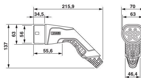
Vehicle connector
