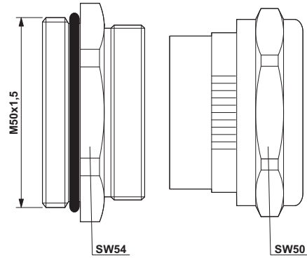
Dimensioned drawing
