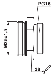
Dimensioned drawing
