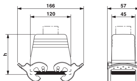
Dimensioned drawing
