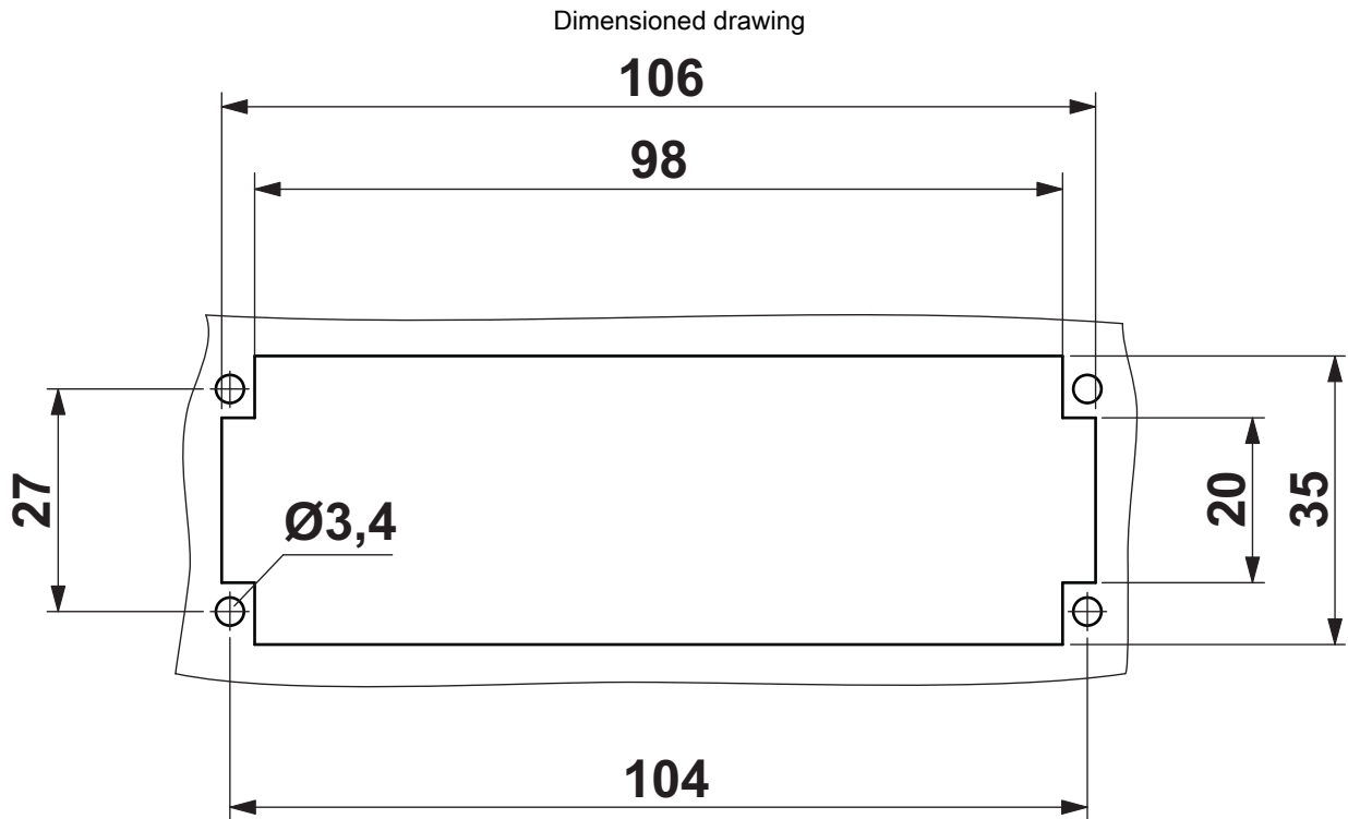
Panel cutout
