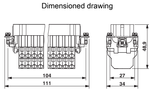
Female insert
